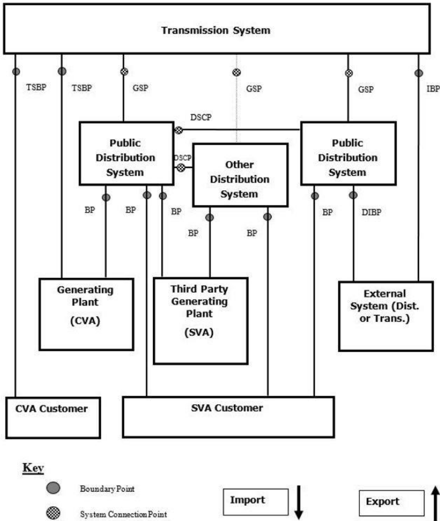
FIGURE 1 IMPORT AND EXPORT ACTIVE ENERGY FLOWS CONVENTION
